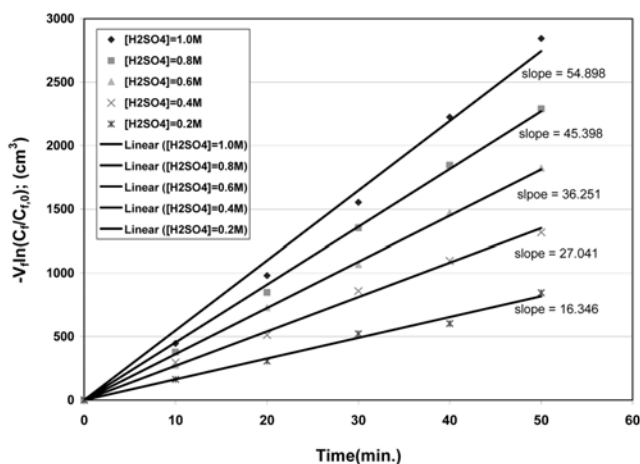
Fig. 10. Plot of -V_f \ln(C_f/C_{f,0}) of As(V) of the feed against time at different H 2 SO 4 acid concentrations.
